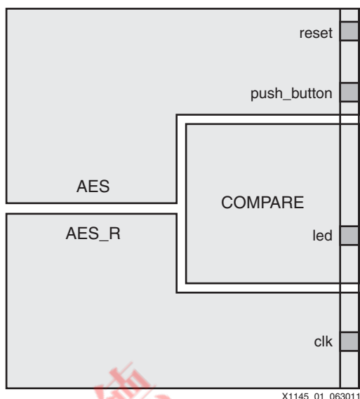
Figure 1: An SCC Solution Using IDF Implementing Two Redundant AES Modules and Compare Logic
