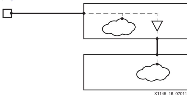
Figure 16: Elimination of a Short by Instantiation of a LUT Buffer
