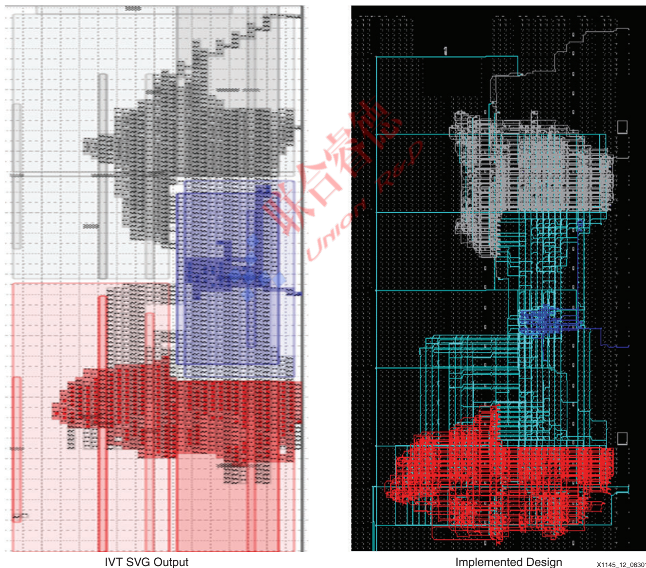
Figure 12: IVT SVG (Left) Run on Reference Design/FPGA Editor View of Same Design (Right)
