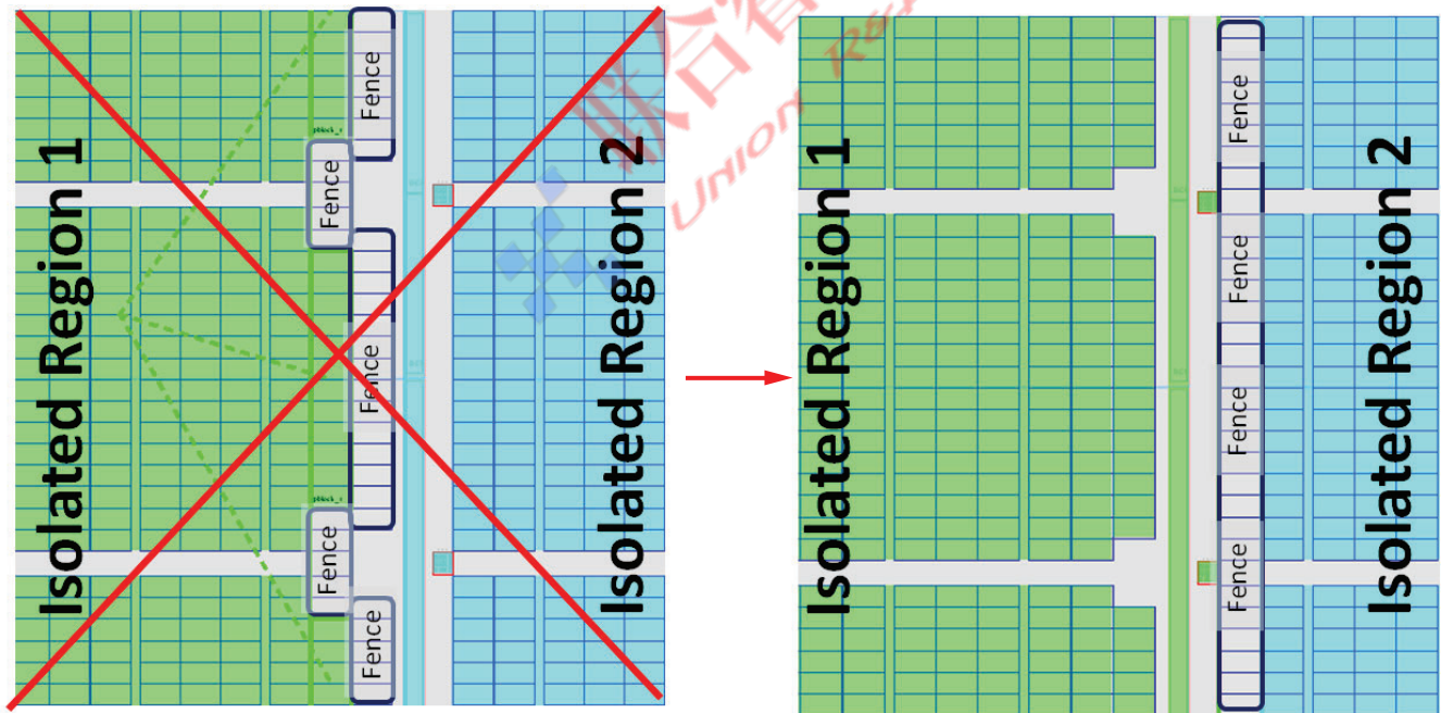
Figure 23: Invalid and Valid Fence Placement Adjacent to Clock Column (DCM/PLL)
