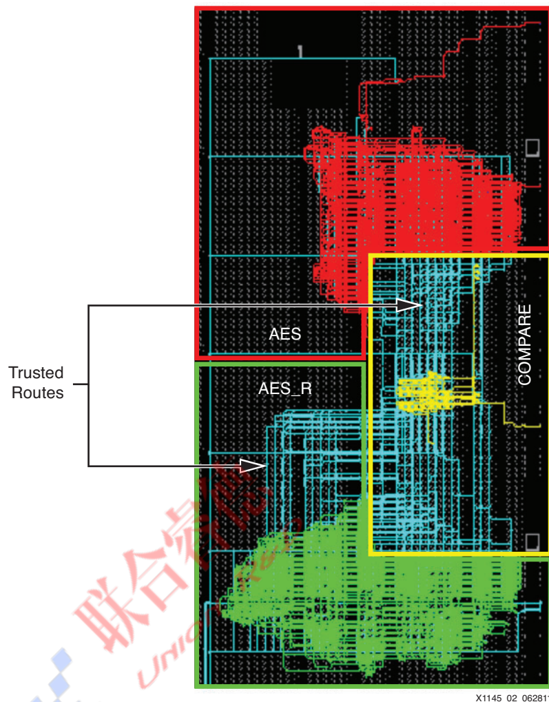
Figure 2: Implemented SCC Solution from Figure 1
