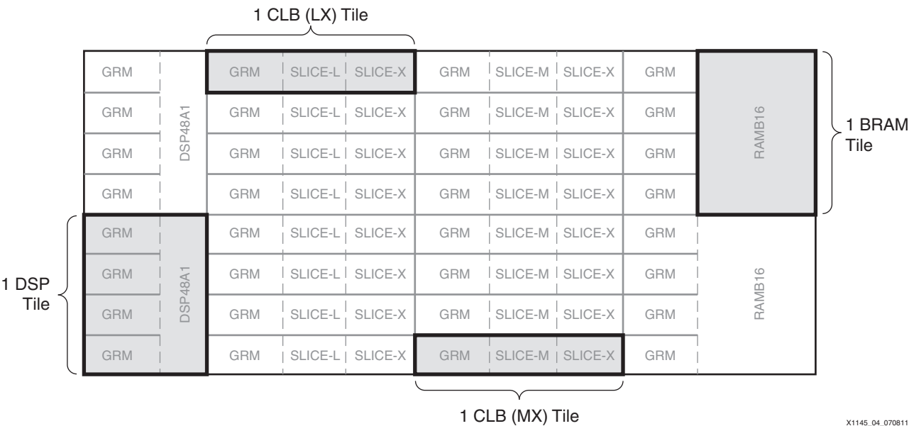
Figure 4: Representation of the Tile-Based Spartan-6 Architecture
